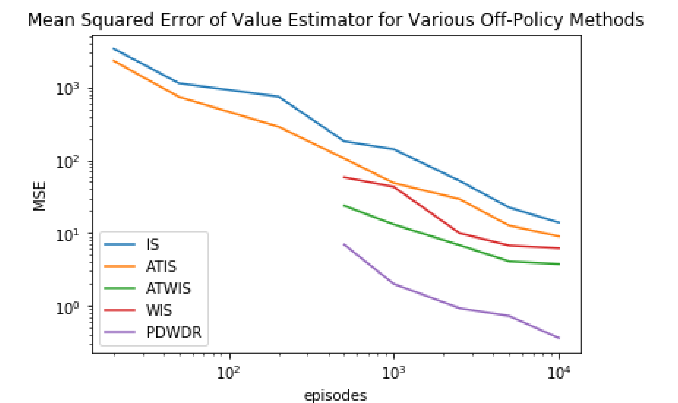
Figure 6: A plot of MSE for various importance sampling methods in a cliff gridworld.
